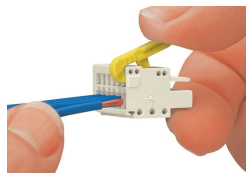
Conductor termination via operating tool (733-191)
